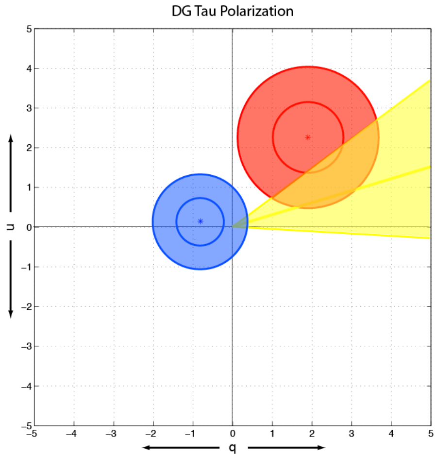
Figure 12.2. Plot in Stokes space of Tamura 850\ \mu\text{m} polarization (red) and SHARP 350\ \mu\text{m} measurement (blue). Stokes q and u are plotted in percent. Circles signify 1\sigma and 2\sigma errorbars. The two measurements do not agree within 2\sigma , which is highly suggestive that there is structure in the polarization spectrum. The yellow region denotes the locus of points that correspond to polarization orientated orthogonally to the plane of the disk (within PA errors). The 850\ \mu\text{m} point appears consistent with this orientation; the 350\ \mu\text{m} measurement is consistent with zero.
