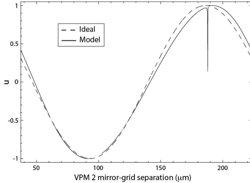
Figure 9.3. VPM Interferogram obtained using a model that treats wire grid performance (Houde et al., 2001). The solid curve shows the model predictions ( u versus grid-mirror separation distance) for the case of grid parameters, wavelength, and incident polarization that match our experiment. The model employs a very narrow bandwidth and assumes regular wire spacing. The spike in the solid curve would be expected to be washed out by the large relative bandwidth of Hertz, and indeed is not observed in Fig. 9.2. The dashed curve shows the idealized sinusoidal interferogram that would be expected for the case of ideal grid and geometric phase delay. In the long wavelength limit, the model curve approaches the idealized curve.
