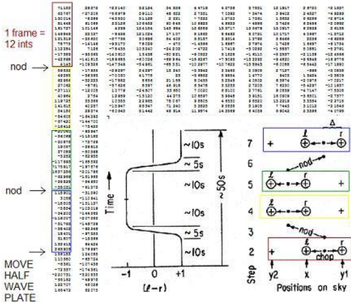
Figure 5.1. Example of data analysis process for single-dish/bolometer applications. Insert taken from Hildebrand et al. (2000). Each column of the sample data represents the output signal (voltage vs. time) of one bolometer, or pixel for either the R or T array. Each number in the column is one “int”, or one demodulated (left-right) signal measurement. A number of ints, or chops , make up one nod. (In the case shown, 12 ints comprise one nod.) We then nod the telescope and take another set of ints/chops. After completing one “nod-pair” (l-r-l), we have collected all of the data for one position of the polarization modulator, here, a HWP.
