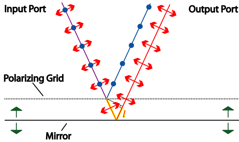
Figure 6.1. A “reflective half-wave plate”. Light incident upon a wire grid is separated into orthogonal polarization components; the component parallel to the wire grid is reflected, while the perpendicular component is transmitted and reflected by a mirror, traveling an extra distance l . When the delay l is set equal to half of the wavelength, this device has the same functionality as a birefringent half-wave plate (HWP)
