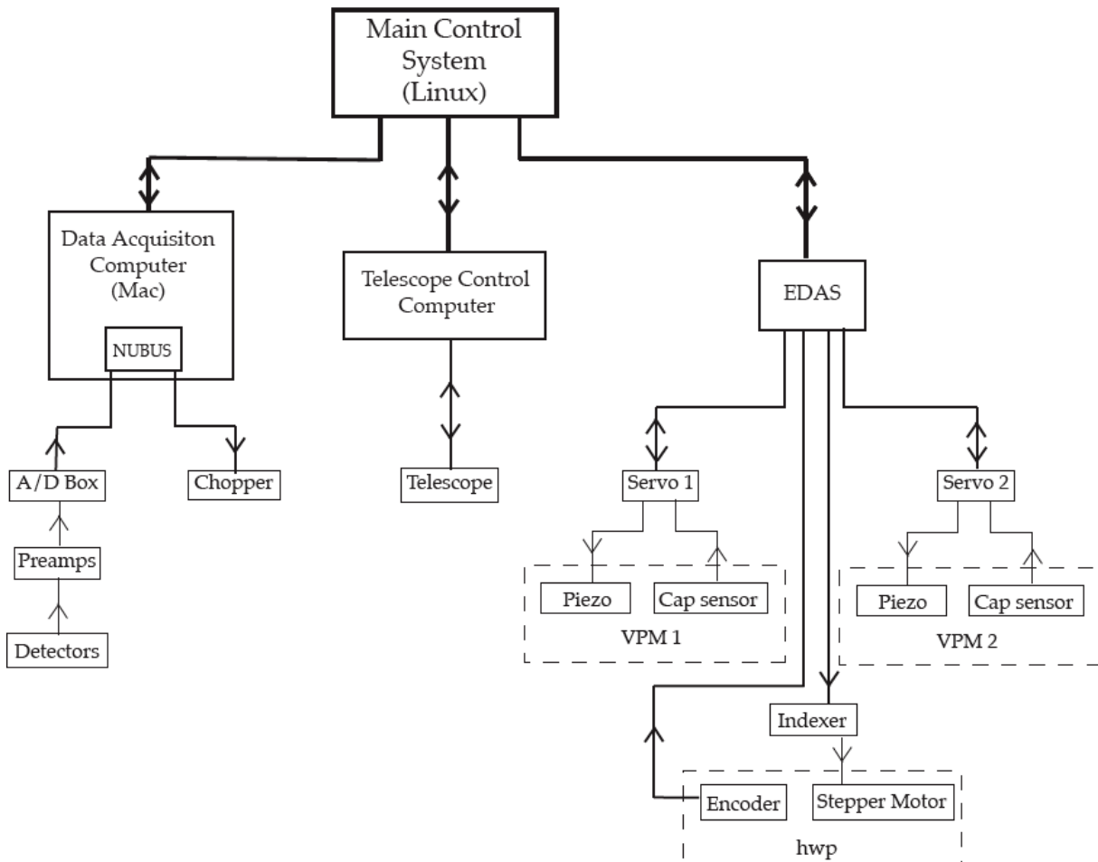
Figure 8.6. Diagram of the Hertz/VPM control electronics. Lines signify paths of communication between components; arrows signify direction. Main control computer communicates with three computers via TCP/IP connections. The data acquisition computer reads demodulated signals from detectors, synchronized by a chopping frequency sent to the secondary mirror. Telescope control computer operates telescope motion and positioning. EDAS controls both the VPMs and the Hertz HWP.
