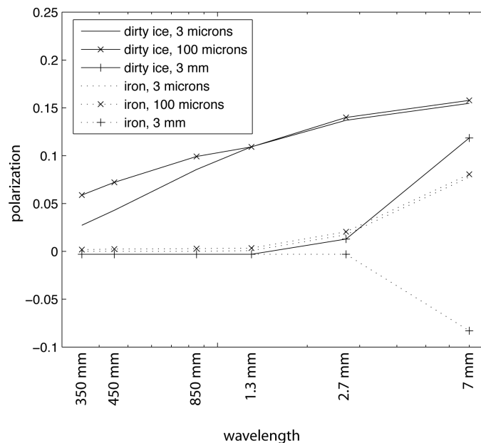
Figure 11.5. Spectrum predictions for polarization by thermally emitting large grains. Each curve represents a single size and type of dust grain; there is no grain size distribution. Polarization is calculated as in section 4.2.2, with the emission coefficients approximated for each axis of the grain by their spherical counterparts. Note that there is no peak in the polarization spectrum; rather, there is a gradual increase with increasing wavelength. The negative polarization point for 3 mm iron grains is due to a decrease in the emission efficiency, as approximated by the plot in Figure 11.1. Curves have slight vertical offset for clarity.
