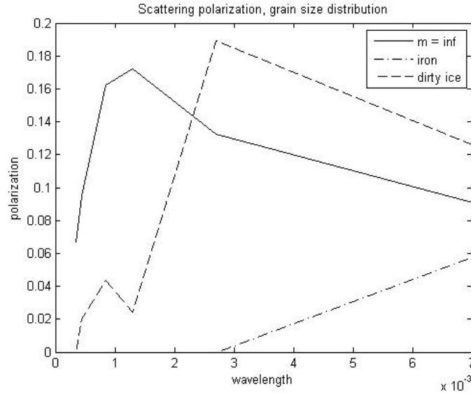
Figure 11.4. Polarization by scattering for both perfect scatterers ( m = \infty ) and grains with absorptive properties. Absorption acts to dampen polarization by scattering at shorter wavelengths. The secondary peak for dirty ice at 850 \mu\text{m} is due to artifacts of our scattering efficiency approximation, and should be ignored.
