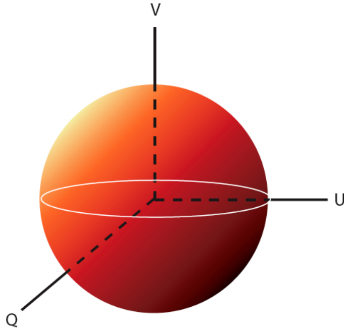
Figure 2.1. The Poincaré Sphere. The Poincaré sphere allows for graphical representation of Stokes parameters. Q , U , and V are the three axes, with I^2 \geq Q^2 + U^2 + V^2 . Points on the surface of the sphere denote fully polarized light, while points inside denote partial polarization. Points lying in the QU plane represent linear polarization.
