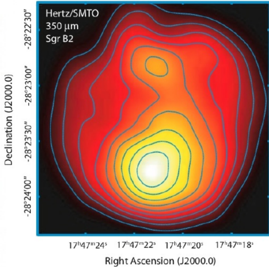
Figure 9.1. 350 \mu\text{m} photometric map of SgrB2, created from VPM files taken with the Hertz/dual-VPM polarimeter. Files were added and smoothed with no flat fielding. Two peaks are shown, \sim 54'' apart, which agree with previous results at this wavelength (Goldsmith et al., 1990). The beam size is 20'' .
