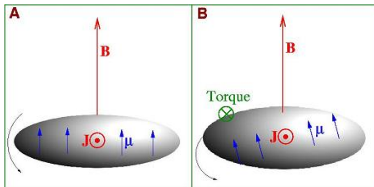
Figure 4.3. Paramagnetic relaxation. The magnetic moment of a spinning dust grain tries to align itself with the surrounding magnetic field. The delay in this alignment creates a torque, damping the rotation having \mathbf{J} perpendicular to \mathbf{B} and leaving only rotation with \mathbf{J} parallel to \mathbf{B} .
