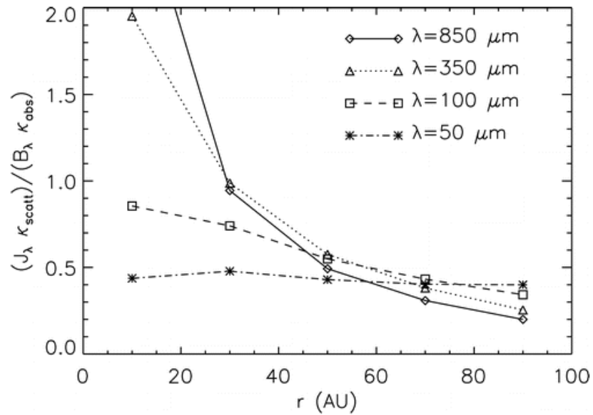
Figure 11.8. Comparison between polarization by scattering and emission, from Cho & Lazarian (2007). Values are plotted as a function of disk radius. Values less than unity signify that thermal emission dominates the flux seen. Values in the submillimeter ( \lambda = 350, 850 \mu\text{m} ) are less than 1, except at the smallest radii. In Section 11.3.2, we learned that polarization at these wavelengths is dominated by the largest disk radii; we thus conclude that polarization by scattering is not dominant in this regime.
