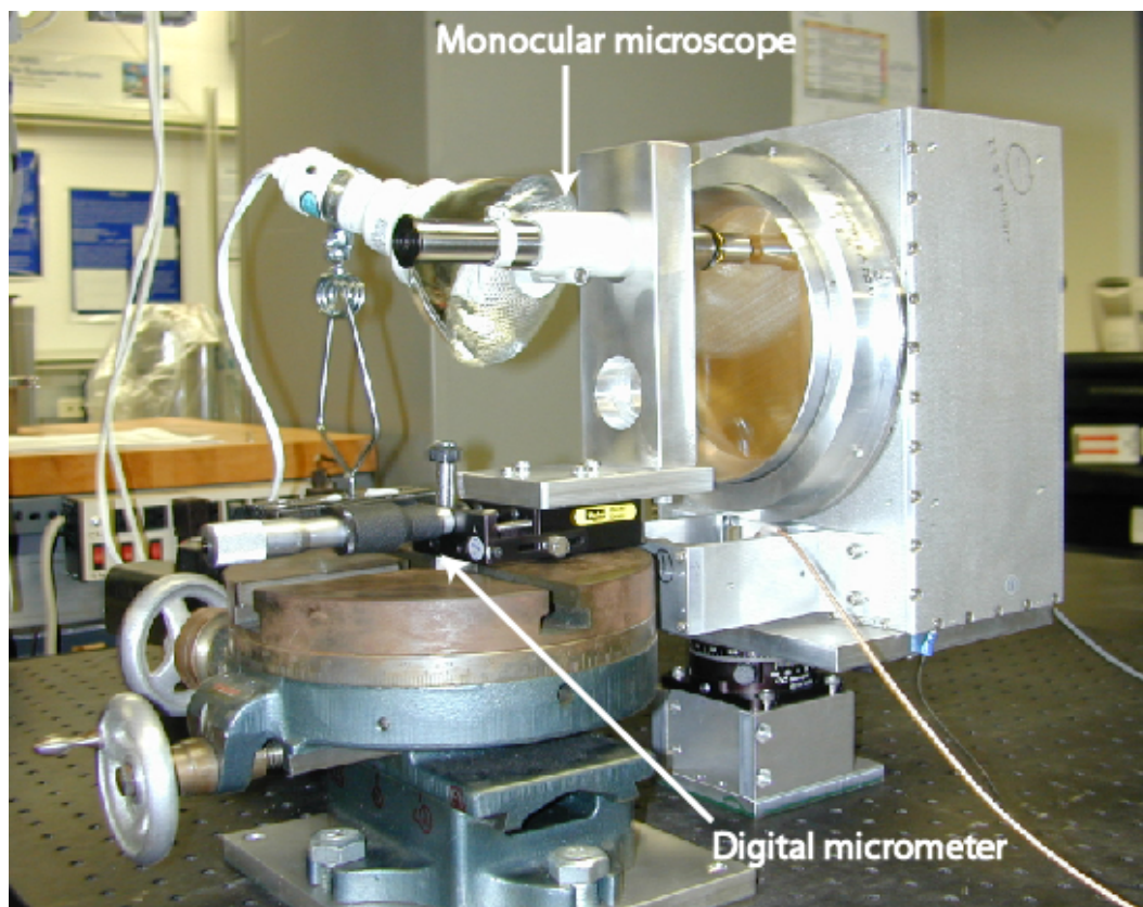
Figure 8.2. Microscope setup for grid-mirror parallelization measurements. The microscope is mounted on a bracket that is moved toward and away from the grid via a linear translation stage that incorporates a digital micrometer. Measurements are made at three points around the edge of the grid.
