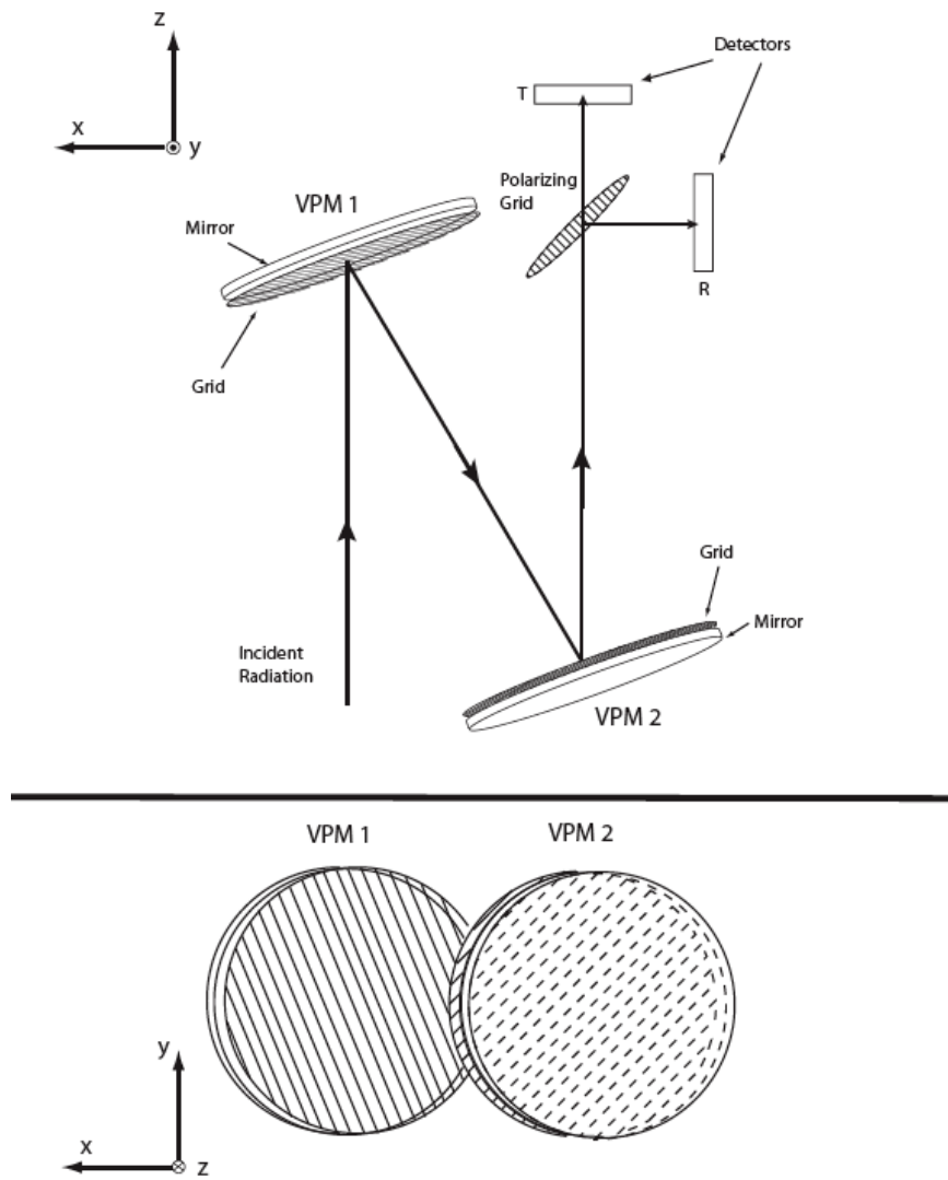
Figure 6.2. Two views of a schematic optical path for a polarimeter incorporating a dual-VPM modulator. The upper panel shows a top view while the lower panel shows the view “seen” by the incoming radiation. The radiation is reflected by two VPMs having their grid wires rotated by 22.5^\circ with respect to one another, and is then incident upon a polarizing grid that splits the beam into orthogonal polarization components directed to detectors R and T (standing for reflected and transmitted). Note that the figure shown above is a general schematic, and is not representative of the actual grid settings and orientations used for the Hertz/VPM experiment.
