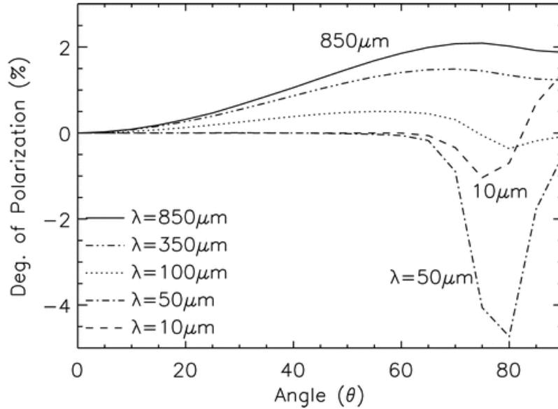
Figure 12.3. Cho and Lazarian (2007) model plot of percent polarization P versus inclination angle for selected wavelengths. Polarization is from disk interior only (interior dominates polarization in submillimeter waveband). The ratio of ( 850 \mu\text{m}/100 \mu\text{m} ) polarization increases drastically with increasing viewing angle, while the ratio for ( 850 \mu\text{m}/350 \mu\text{m} ) changes only slightly.
