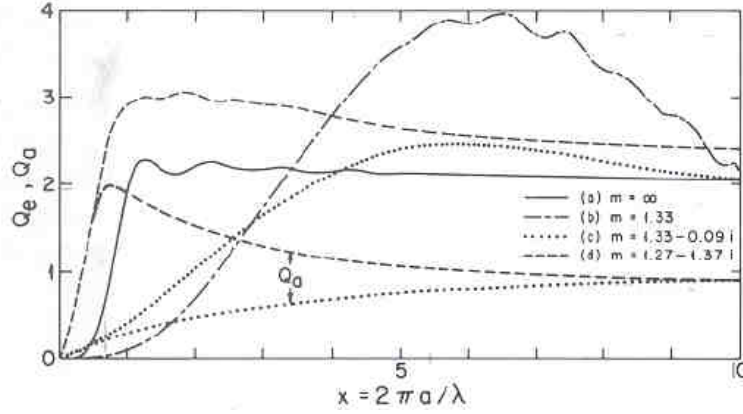
Figure 11.1. Extinction ( Q_e ) and absorption ( Q_a ) efficiencies as a function of inverse wavelength for dust grains of different complex refractive indices, from Spitzer (1978). Our toy models employ these curves. Scattering efficiency was calculated by subtracting Q_{abs} from Q_{ext} . The grains are spherical with radius a .
